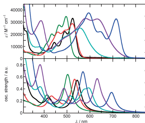
Figure 3. UV/vis absorption spectra of tetrachlorotetraamino-PDIs: 6 a (red), 7 (olive), 8 (black), 9 (cyan), 10 a (purple), and biscarbazolo[2,3- b ]carbazole diimides 11 a (blue) in chloroform (top), and comparison with TDDFT/PBE1PBE/6-31G*/PCM computed spectra not including vibronic structures (bottom).
