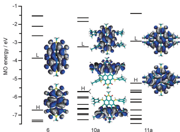
Figure 4. Energies and shapes of PBE1PBE/6-31G*/PCM frontier orbitals (HOMO and LUMO) of model Br 4 Cl 4 -PDI 6 , tetrachlorotetraamino-PDI 10a , and biscarbazolo[2,3- b ]carbazole diimides 11a .
