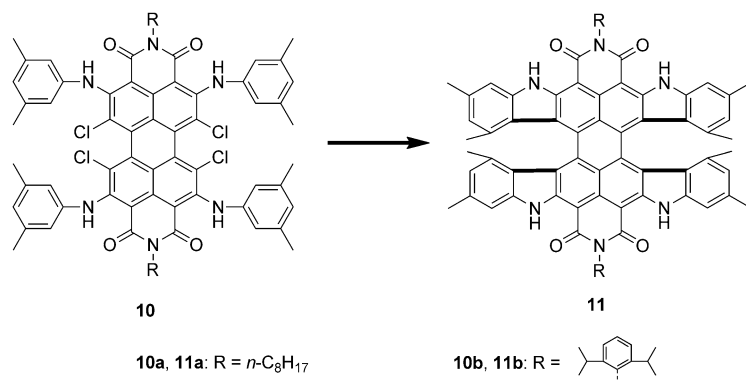
Scheme 2. [\text{Pd}_2(\text{dba})_3] , \text{P}(\text{tBu})_3 , \text{K}_3\text{PO}_4 , 1,4-dioxane, reflux, argon, 11 a (45%), 11 b (32%). dba = dibenzylideneacetone.
